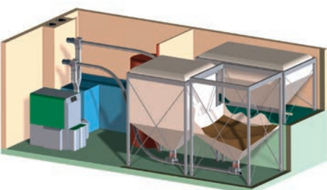
2 Flexilo® MAXI and 1 Flexilo® Through with direct feed to a 180 kW boiler
