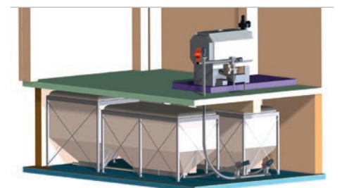
4 Flexilo® Through with direct feed to cross spiral
