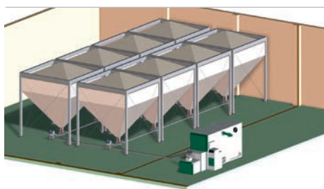
Flexilo® MAXI - storage capacity 120 t - 1000 kW
