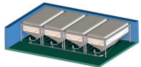
4 Flexilo® Through with transfer hopper to cross spiral with suction point
